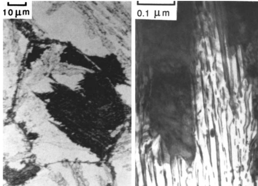
Fig. 11.4 Microstructure of the so-called 'pearlitic bainite', which is really just a pearlite with alloy carbide (in this case M_7C_3 ) instead of cementite: (a) light micrograph; (b) transmission electron micrograph.
