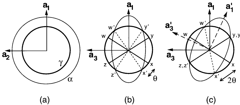
Fig. 2.22 (a) and (b) show the effect of the Bain strain on austenite, which when undeformed is represented as a sphere of diameter wx = yz in three-dimensions. The strain transforms it to an ellipsoid of revolution. (c) shows the invariant-line strain obtained by combining the Bain strain with a rigid body rotation.
