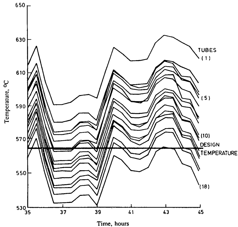
Fig. 4.10 Illustration of the variation in the temperature at different locations on a particular component ('reheater drum') of a 500 MW power station (Cane and Townsend, 1984).
