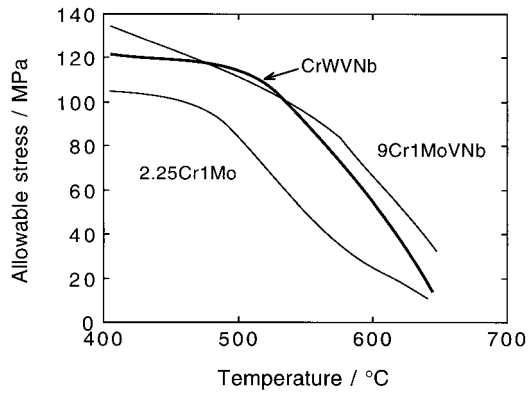
Fig. 12.24 Comparison of the allowable stress, as a function of temperature, for the tungsten-strengthened steel, 2\frac{1}{4}\text{Cr1Mo} and a 9\text{Cr1Mo} martensitic steel. After Komai et al. (1999).
