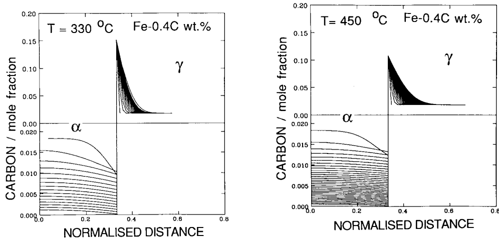
Fig. 6.19 The concentration profiles that develop in ferrite and austenite during the partitioning of carbon from supersaturated bainite (Fe-0.4C wt%, plate thickness 0.2 \mu\text{m} ). (a) 330^\circ\text{C} , the time interval between the concentration contours in each phase being 0.094 \text{ s} . (b) 450^\circ\text{C} , the corresponding time interval is 0.007 \text{ s} . (Mujahid and Bhadeshia, 1992).
