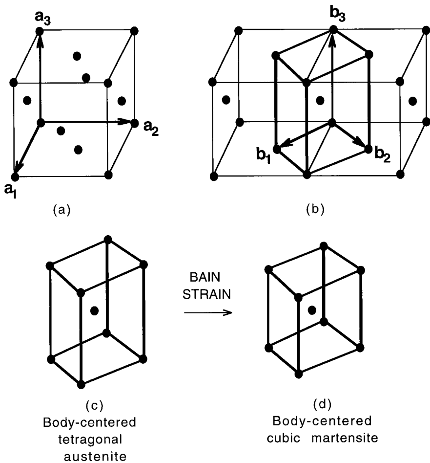
Fig. 2.17 (a) Conventional FCC unit cell of austenite, with basis vectors \mathbf{a}_1, \mathbf{a}_2, \mathbf{a}_3 . (b) Relation between the FCC and body-centered tetragonal cell ( \mathbf{b}_1, \mathbf{b}_2, \mathbf{b}_3 ) of austenite. (c,d) Bain Strain deforming the austenite lattice into a BCC martensite lattice.
