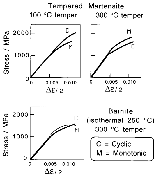
Fig. 12.17 Data illustrating the differences between the cyclic and monotonic yield behaviours for tempered martensite and bainite in 300M steel (Ritchie, 1977a).
