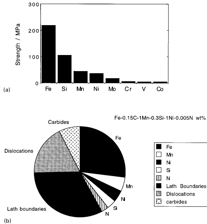
Fig. 12.1 The tensile yield strength of bainite at 25 °C and a strain rate of 0.0025 s -1 : (a) typical solid solution strengthening contributions per wt% of solute in ferrite; the intrinsic strength of pure iron is also included (data from Leslie, 1982); (b) estimated contributions to the strength of a fully bainitic sample.
