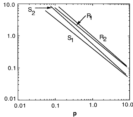
Fig. 6.13 Dependence of Trivedi's functions S_1 , S_2 , R_1 and R_2 on the Péclet number p .
