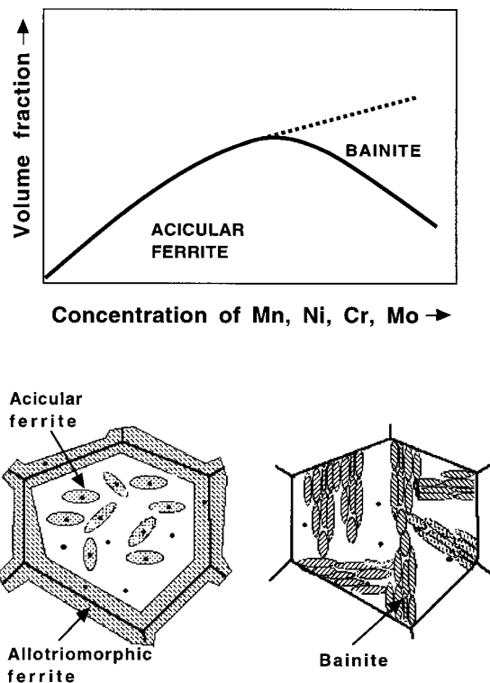
Fig. 10.16 Schematic illustration of the mechanism by which the presence of allotriomorphic ferrite at the austenite grain surfaces induces a transition from a bainitic to acicular ferrite microstructure.
