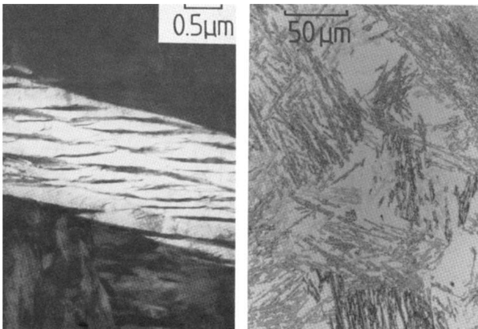
Fig. 13.21 (a) Transmission electron micrograph of bainitic ferrite plates separated by films of stable austenite. (b) Optical micrograph showing the large blocks of austenite left untransformed.
