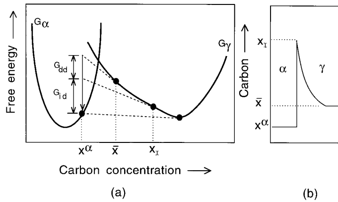
Fig. 6.22 (a) Constant temperature free-energy curves showing the quantities G_{dd} and G_{id} for the case where the interface compositions are as illustrated in (b). Note that the net free energy available for interfacial motion after allowing for strain energy and interface energy contributions is \Delta G , which is the sum of the two dissipations G_{dd} and G_{id} .
