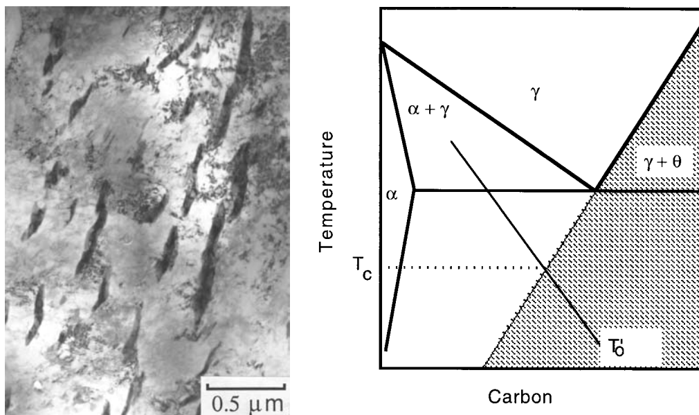
Fig. 3.1 (a) Distribution of cementite particles between the ferrite platelets in upper bainite (AISI 4340 steel). (b) Thermodynamic condition which must be satisfied before cementite can precipitate from austenite.
