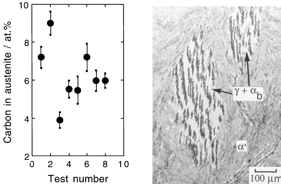
Fig. 3.4 The nonuniform distribution of carbon in the residual austenite associated with bainitic ferrite. (a) Direct measurements of the carbon concentration using an atom-probe; Fe-0.39C-2.05Si-4.08Ni wt%, isothermally transformed at 340°C for 10 h (Bhadeshia and Waugh, 1981). (b) Rim of austenite retained around a sheaf of bainite in Fe-0.81C-1.98Si-3Mn wt% steel, where the carbon concentration is expected to be largest.
