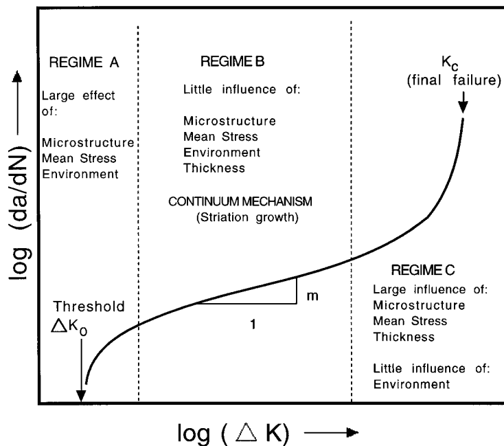
Fig. 12.15 Schematic illustration of the variation in fatigue crack growth rate as a function of the stress intensity range (after Ritchie, 1979.)
