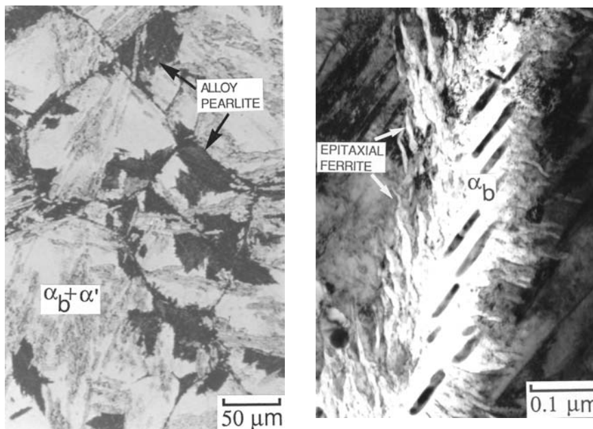
Fig. 4.5 The decomposition of residual austenite once the bainite reaction has stopped. (a) Pearlite colonies; (b) ferrite growing epitaxially from bainite plates.
