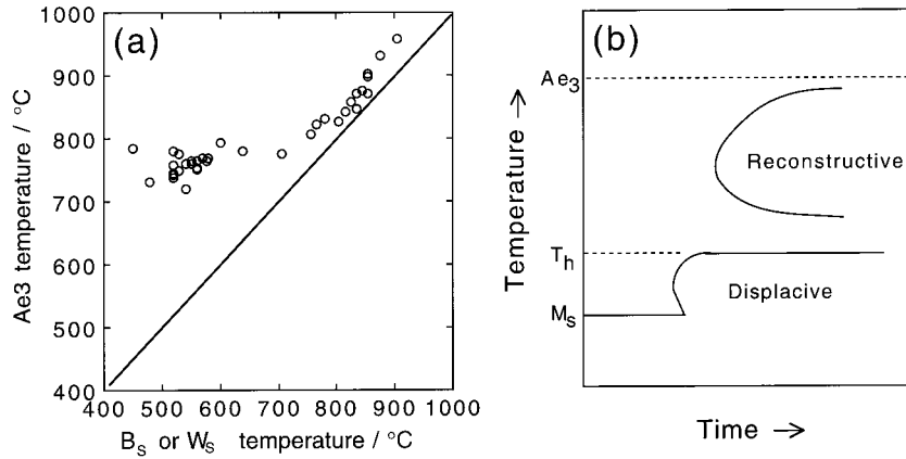
Fig. 6.3 (a) The variation of the Widmanstätten ferrite-start and bainite-start temperatures as a function of the A_{e3} temperature of the steel concerned (Ali, 1990). (b) Schematic TTT diagram illustrating the two C-curves and the T_h temperature.
