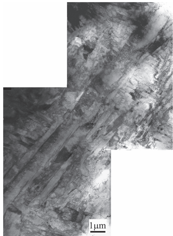
Figure 7. TEM micrograph from Alloy 1 showing a martensite / bainite microstructure.
