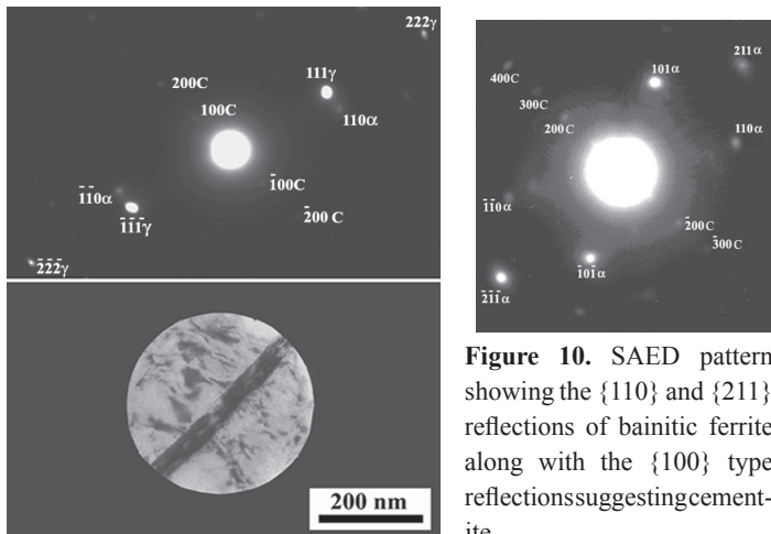
Figure 9. SAED pattern (above) corresponding to the bright field image of the SA aperture over the dark film (below). Results show the {111} and {222} spots from austenite, the {110} spots from ferrite and the {100} type spots suggesting cementite.
