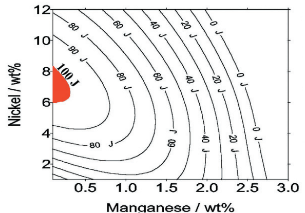
Figure 1. Contour plot showing the predicted behaviour of weld toughness at -40\text{ }^{\circ}\text{C} as a function of Mn and Ni concentration.
