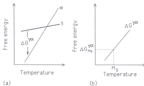
Fig. 9: (a) Difference in the free energies of austenite and martensite of the same chemical composition as a function of temperature. (b) Formation of martensite when the driving force achieves a critical value.
