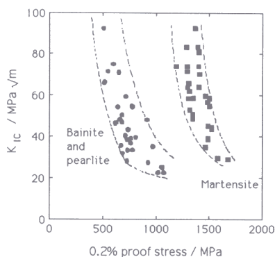
Fig. 2: Fracture toughness K_{IC} as a function of the strength [13]
