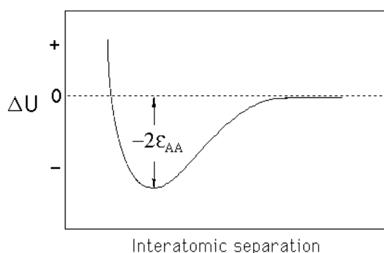
Fig. 3: Curve showing schematically the change in energy as a function of the distance between a pair of A atoms. -2\epsilon_{AA} is the binding energy for the pair of atoms. There is a strong repulsion at close-range.
