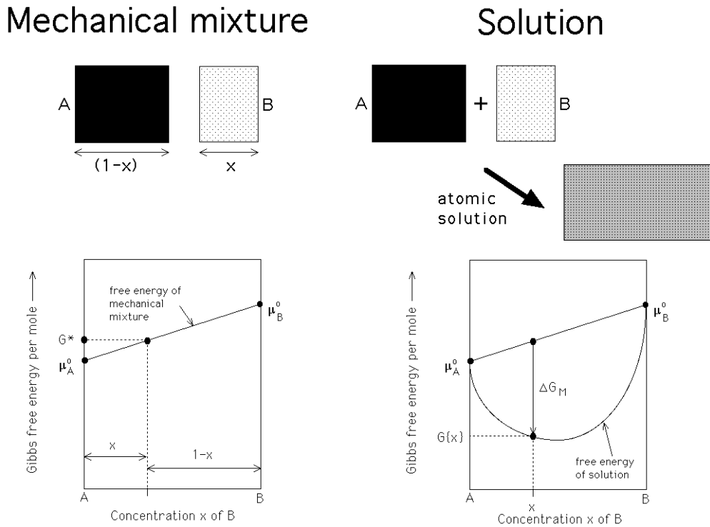
Fig. 1: (a) The free energy of a mechanical mixture, where the mean free energy is simply the weighted mean of the components. (b) The free energy of an ideal atomic solution is always lower than that of a mechanical mixture due to configurational entropy.
