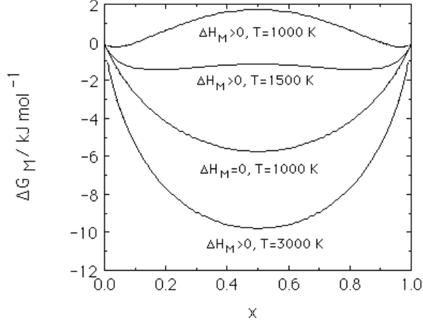
Fig. 5: The free energy of mixing as a function of concentration and temperature in a binary solution where there is a tendency for like atoms to cluster. The free energy curve for the ideal solution ( \Delta H_M = 0 ) is included for reference.
