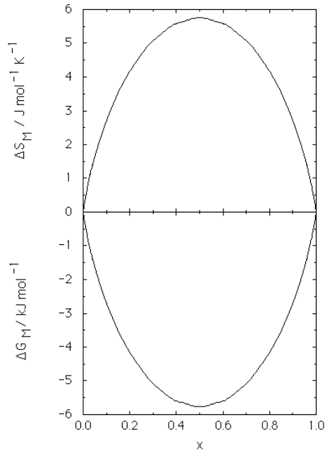
Fig. 2: The entropy of mixing and the free energy of mixing as a function of concentration in an ideal binary solution where the atoms are distributed at random. The free energy is for a temperature of 1000 K.
